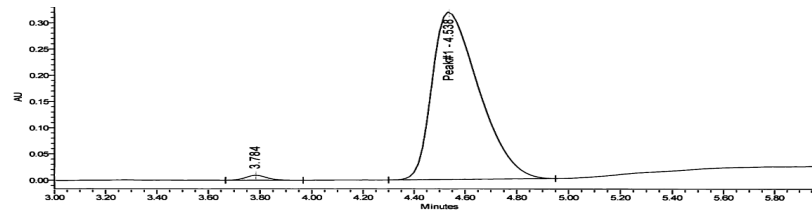
HPLC-UV Chromatogram
