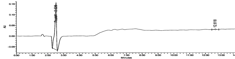
HPLC-UV Chromatogram
