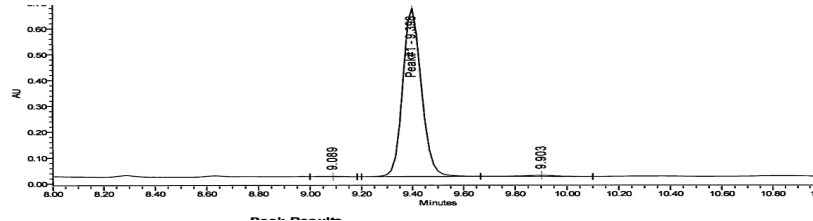
HPLC-UV Chromatogram
